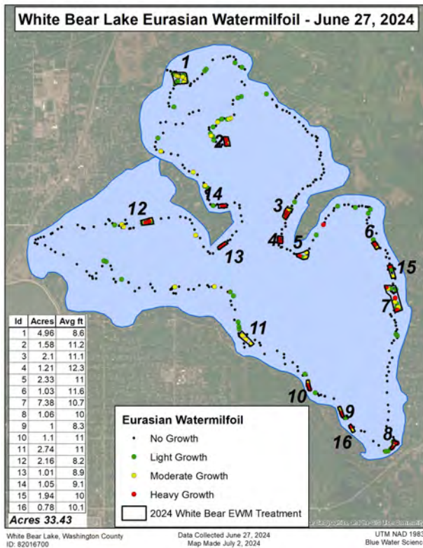
Figure 1. [left] EWM delineation with treatment polygons for June 27, 2024. [right] EWM assessment on August 20, 2024 found mostly light to moderate EWM growth. Key: green dots = light growth, yellow dots = moderate growth, red dots = heavy growth, and black dots = no EWM growth.
